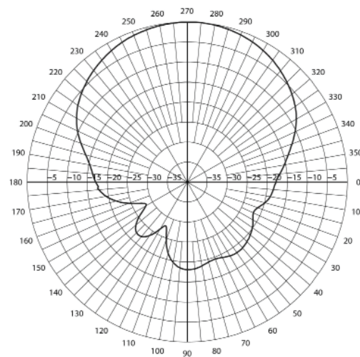
MP9026 Azimuth Cut
