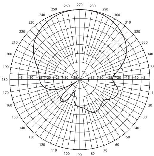
MP9027XFPTNF Elevation Cut
