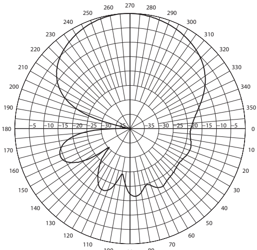
MP8066XFPTNF Elevation Cut
