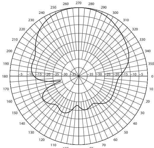
MP8066XFPTNF Azimuth Cut
