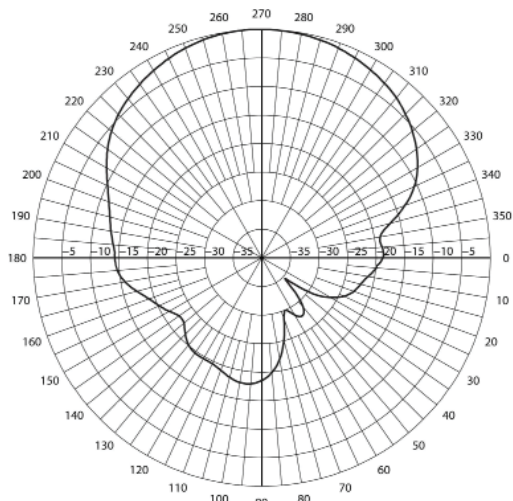
MP9026 Elevation Cut
