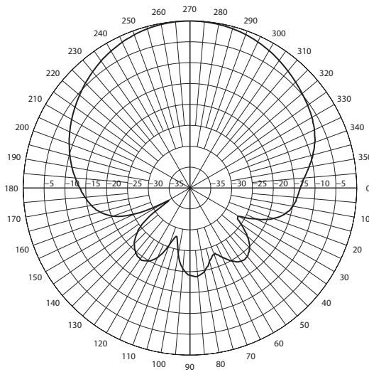
MP9027XFPTNF Azimuth Cut
