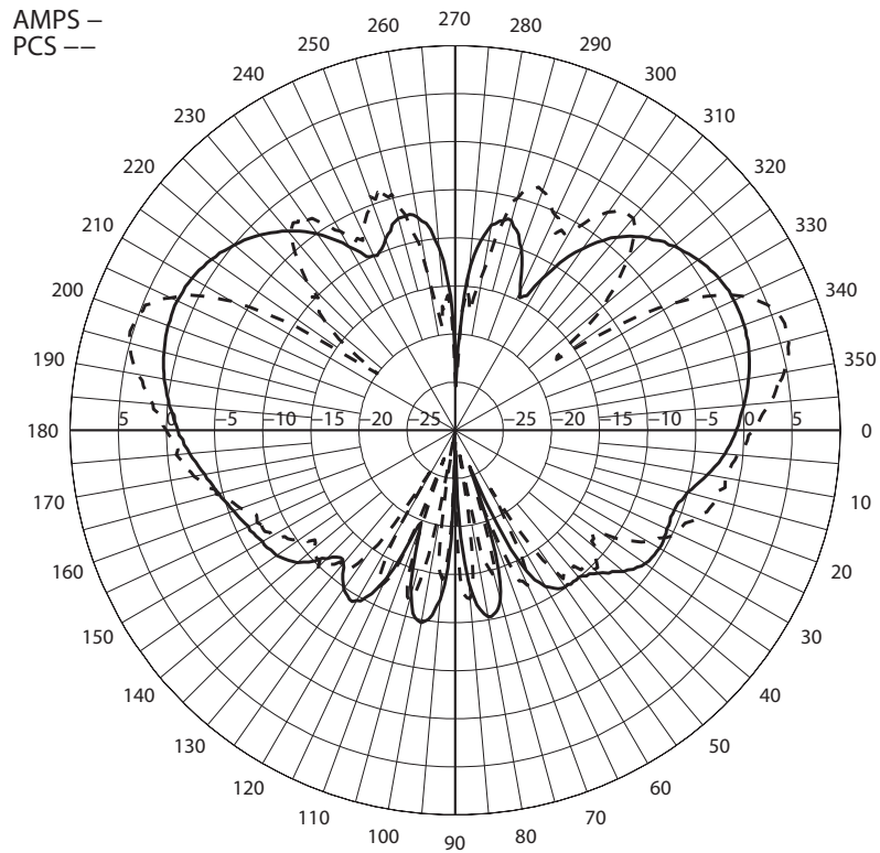
BMMG824/1900 Elevation Cut
