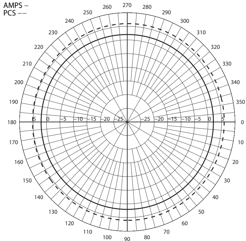
BMMG824/1900 Azimuth Cut
