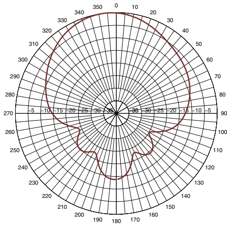
1850 MHz E-Plane Pattern
