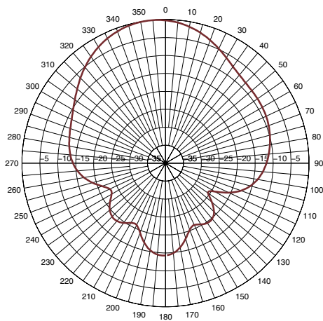
2300 MHz E-Plane Pattern
