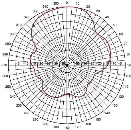
2600 MHz E-Plane Pattern
