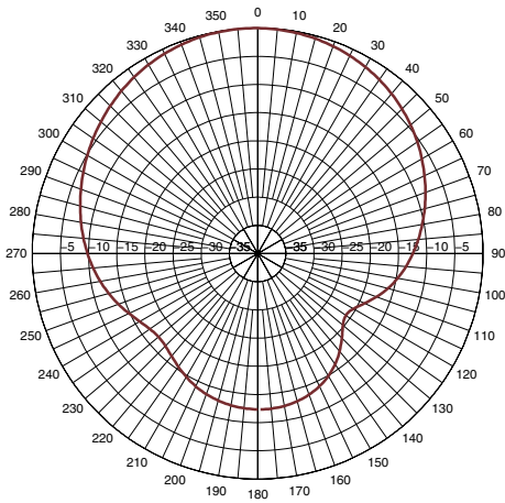
800 MHz E-Plane Pattern
