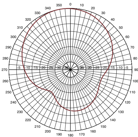
900 MHz E-Plane Pattern
