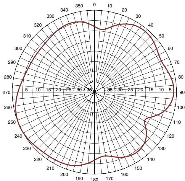
1710MHZ_AZ
