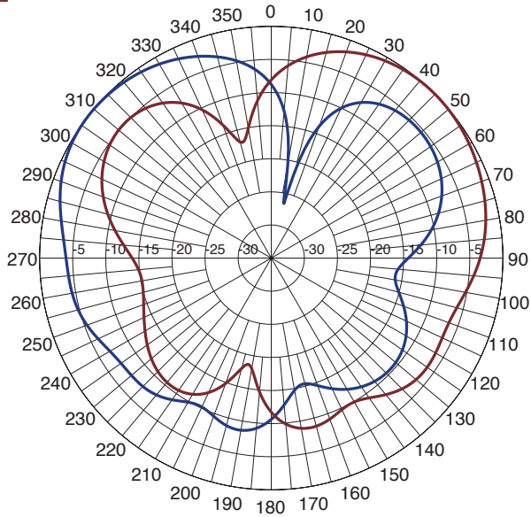
Elevation Pattern at 698MHz
