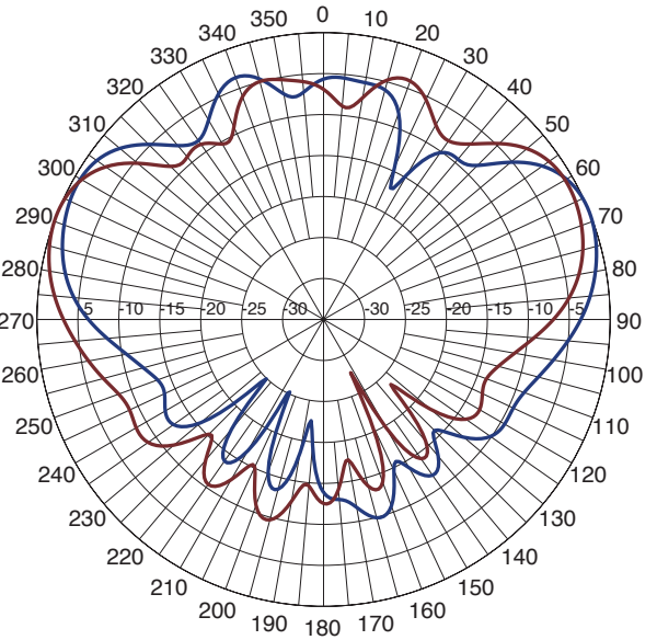
Elevation Pattern at 1850MHz
