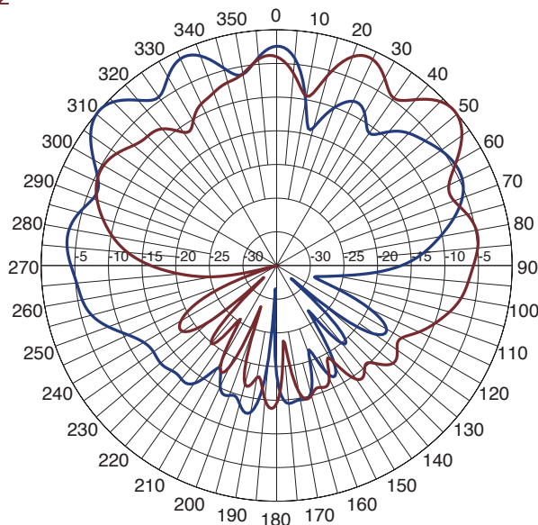
Elevation Pattern at 2600MHz
