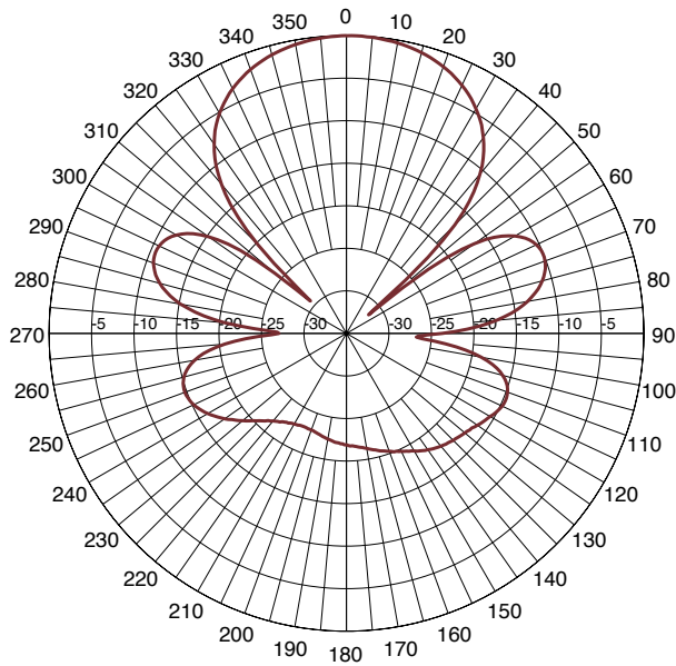
Port 2 Elevation Pattern at 757MHz
