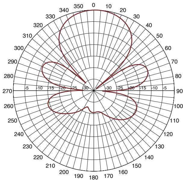
Port 1 Azimuth Pattern at 757MHz
