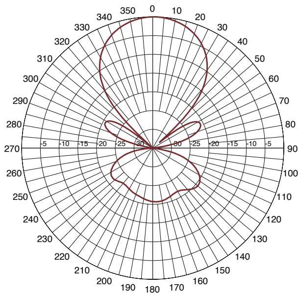
Port 2 Azimuth Pattern at 757MHz
