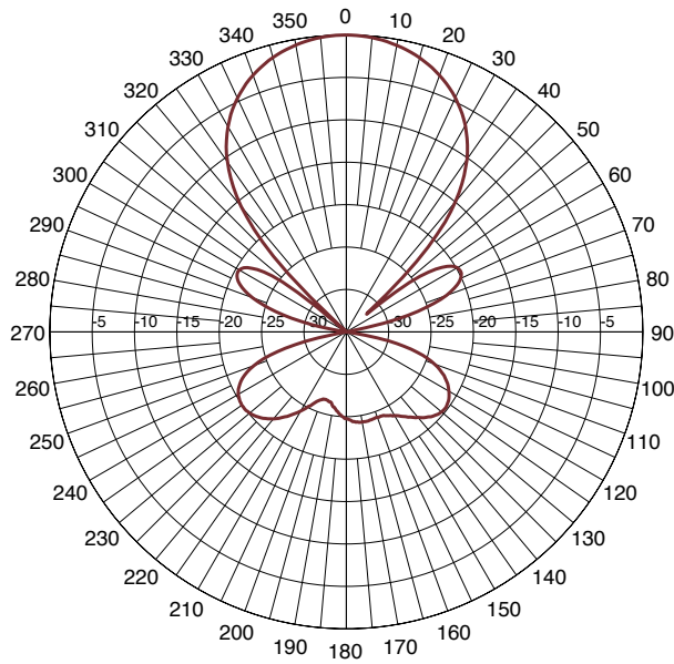
Port 1 Elevation Pattern at 757MHz
