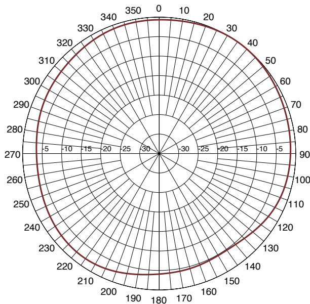
Azimuth Pattern at 5400MHz
