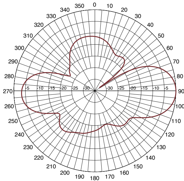
Elevation Pattern at 5400MHz
