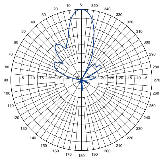
Elevation Pattern at 2240 MHz
