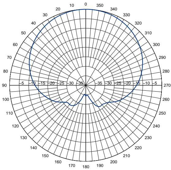
Azimuth Pattern at 2240 MHz
