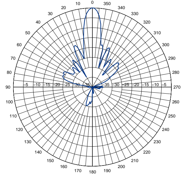
Elevation Pattern at 5500 MHz
