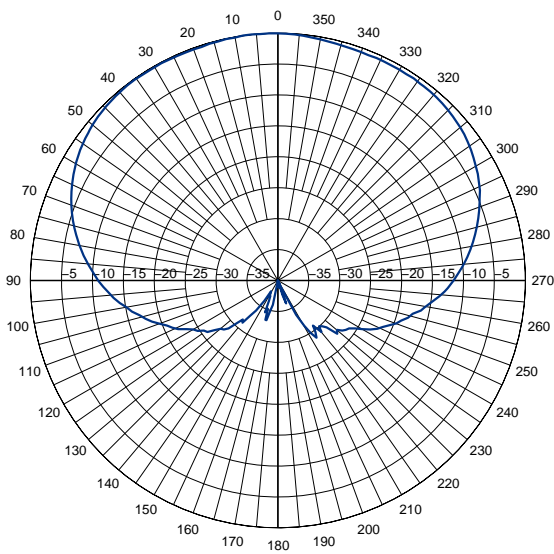
Azimuth Pattern at 5500 MHz
