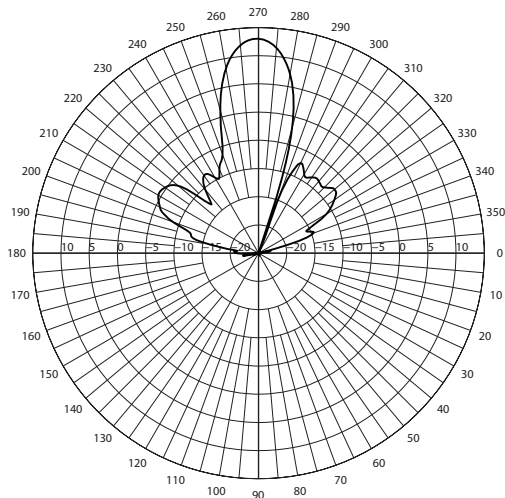
MSP24013MB Elevation Pattern
