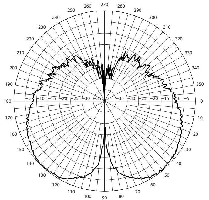
UFDD24580303PT Elevation Cut at 5 GHz
