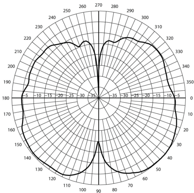
UFOD24003PT Elevation Cut
