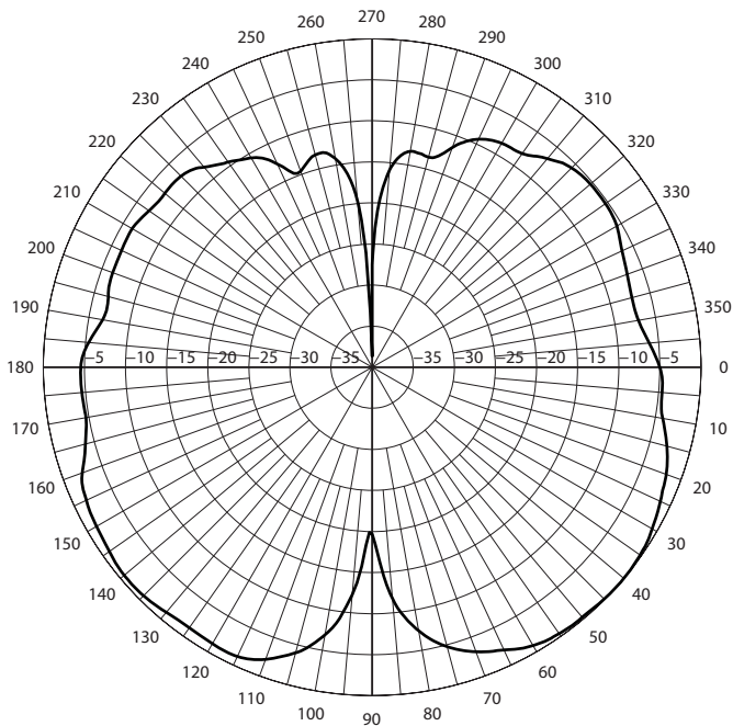
UFDD24580303PT Elevation Cut at 2.4 GHz
