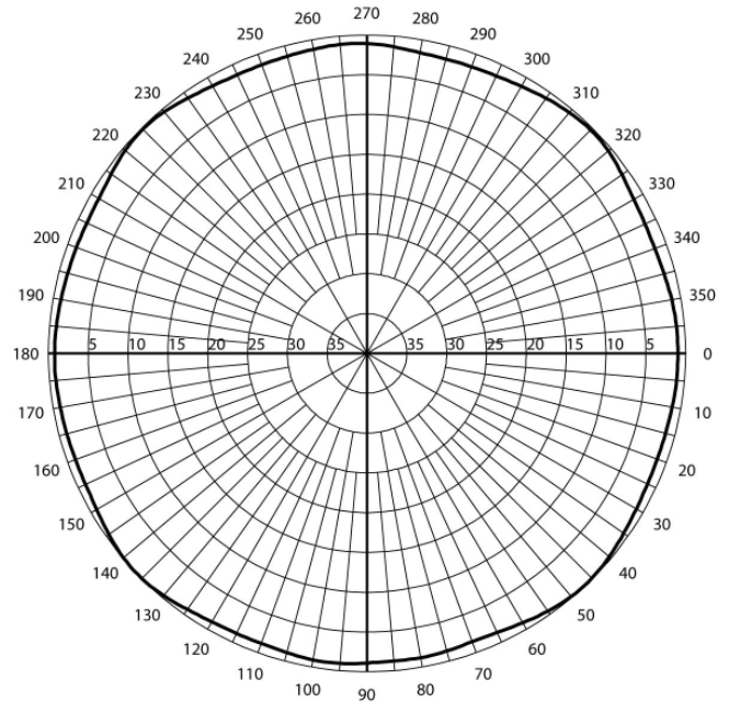
UFOD24003PT Azimuth Cut
