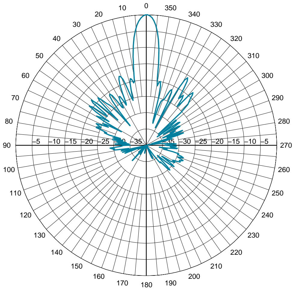
WISP4959018MBV Elevation Cut
