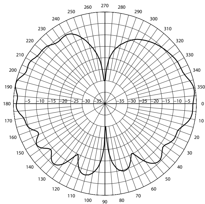
Azimuth Cut at 2.4 GHz
