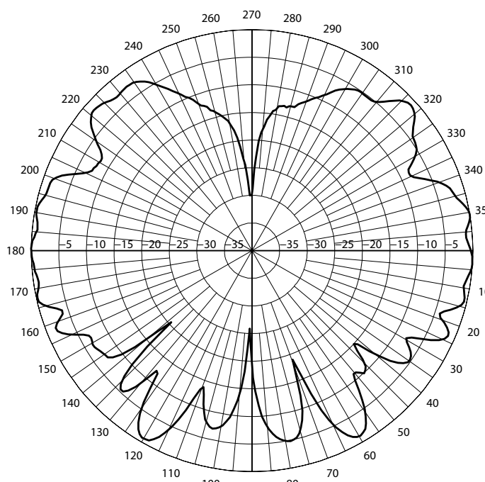
Elevation Cut at 5.0 GHz
